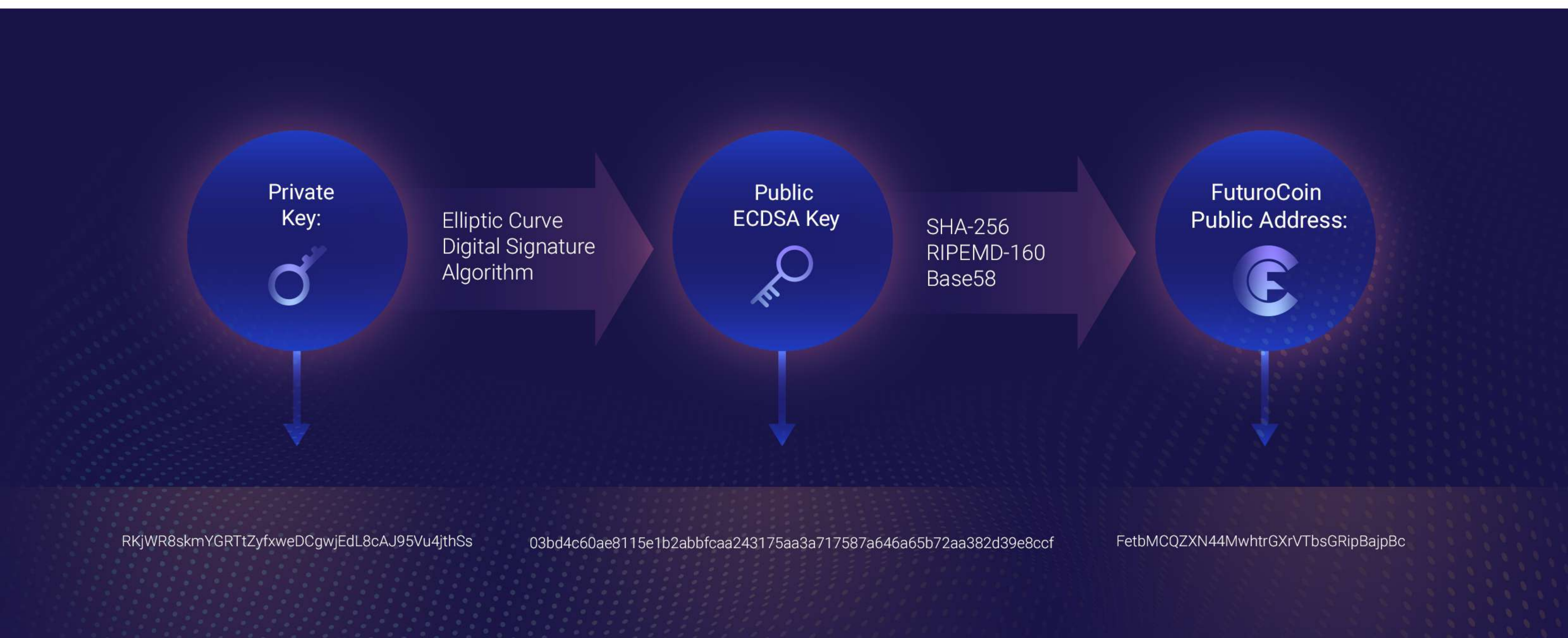
(Figure 1 Public address generation algorithm)
